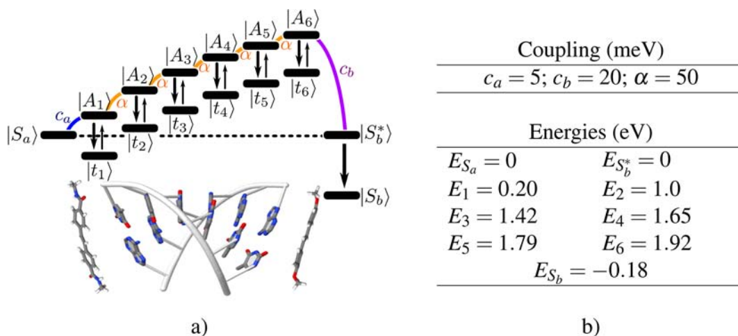
Figure 1. Schematic representation of the model used to study the hole propagation across the hairpin 6 (a) and parameters of the model (b). Starting from the hole donor |S_a\rangle , the hole propagates on the states |A_n\rangle . The hole density can be partially localized on the |t_n\rangle states and possibly thermally activated later on. The hole density can eventually reach the hole acceptor excited state |S_b^*\rangle before the final localization of the hole on the ground state of acceptor |S_b\rangle occurs.
